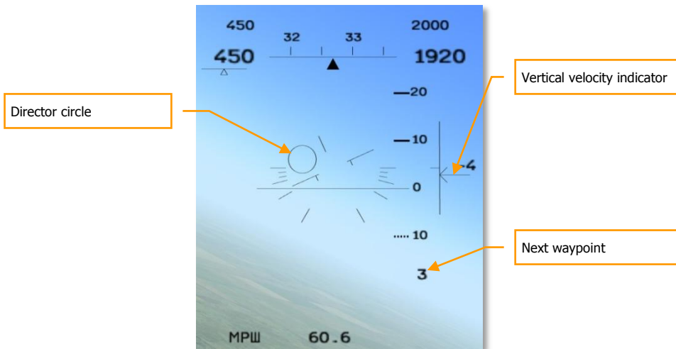
Figure 22: MPW (ENROUTE) Navigation Sub-Mode
