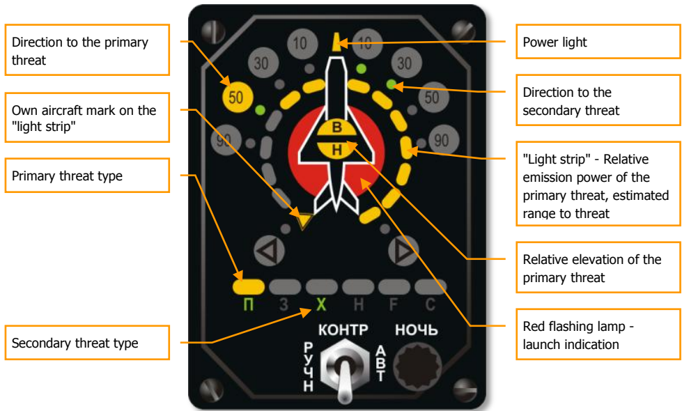
Figure 17: "Beryoza" SPO-15LM indicator
