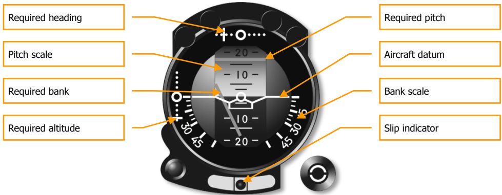
Figure 10: Attitude Direction Indicator (ADI)
