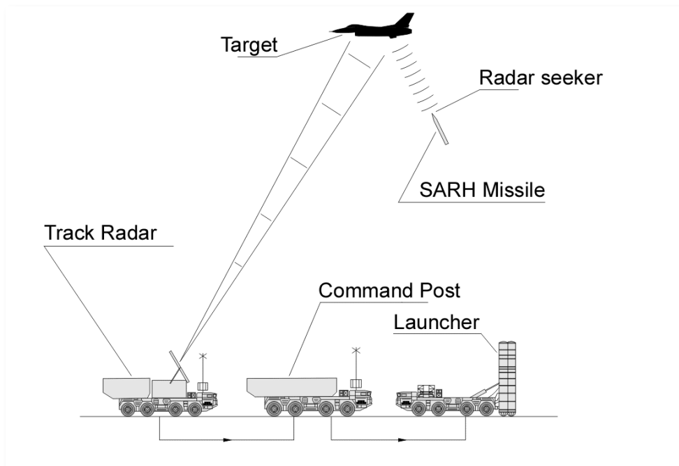
13-3: Semi-active guidance
