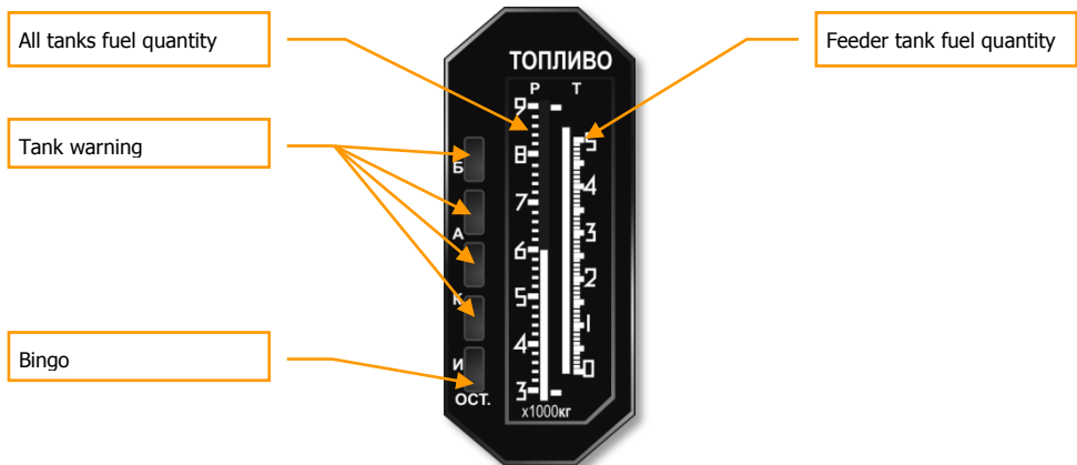
3-46: Fuel Quantity Indicator
