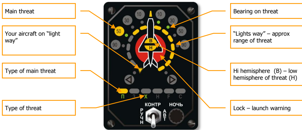
3-15: RWS indicator
