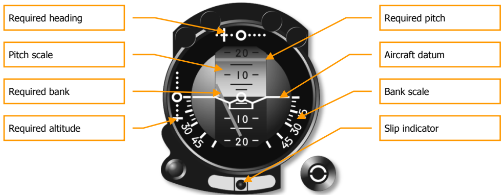
3-41: Attitude Director Indicator (ADI)
