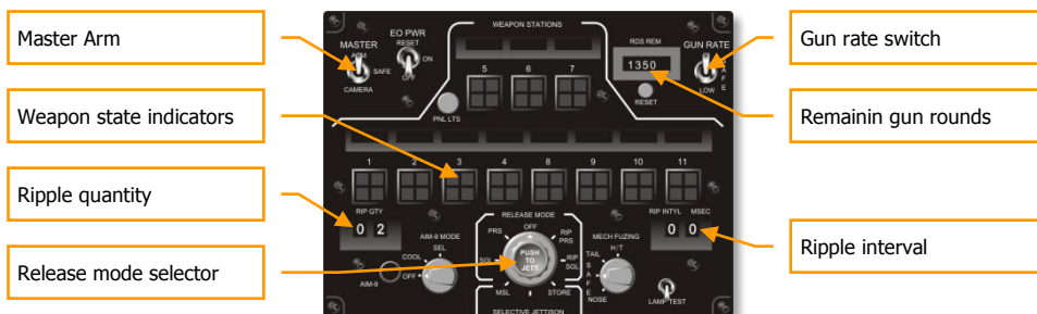
4-61: Armament Control Panel
