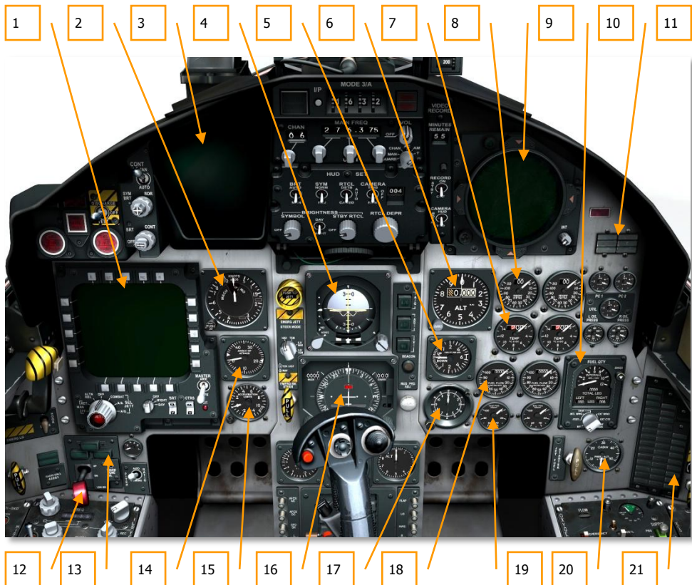
4-1: F-15C instrument panel
